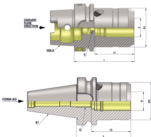
Technical Information : Hydraulic Expansion Chucks (Heavy Duty Series)
