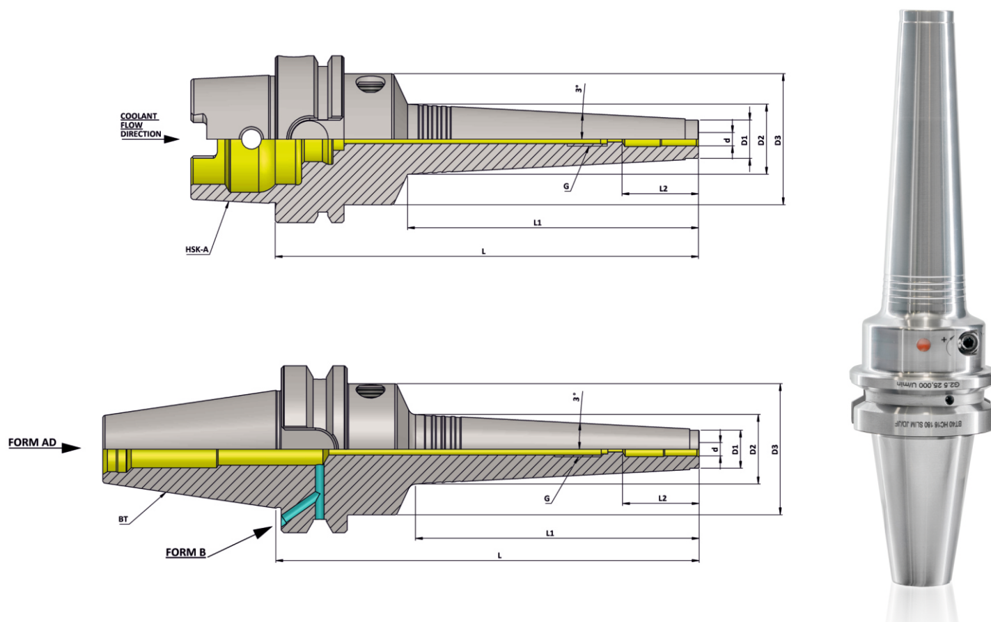
Technical Information : Hydraulic Expansion Chucks (Slim 3° Series)
