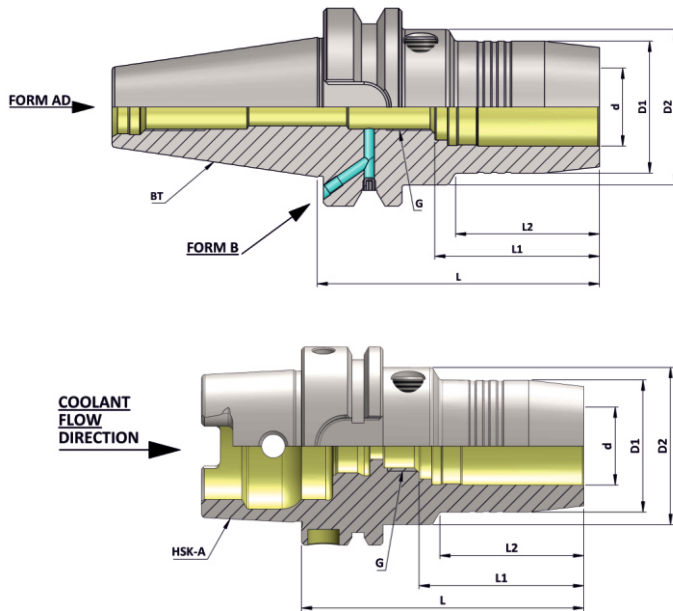
Technical Information : Hydraulic Expansion Chucks (Standard Series)
